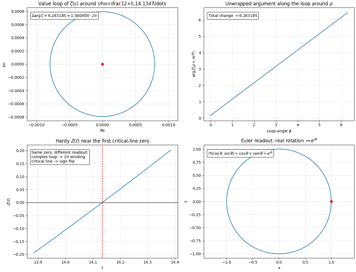
Figure 3: Numerical readout: local value loop of \zeta around the first critical-line zero, unwrapped argument change, Hardy sign flip, and Euler readout as real rotation viewed through the complex map \Pi(x, y) = x + iy .
